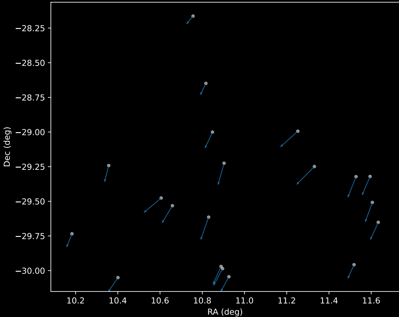
APOGEE DR17 Cluster 20 Proper Motion Vectors (n=20)
