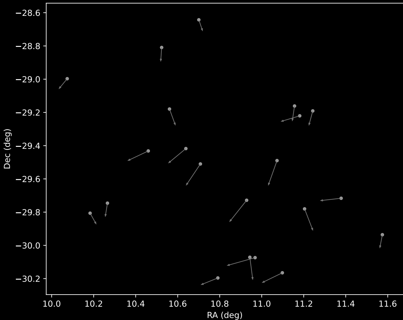
APOGEE DR17 Cluster 14 Proper Motion Vectors (n=21)
