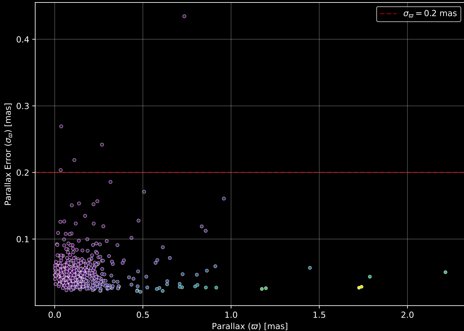
APOGEE DR17 Field: [002-04] Parallax Quality (n= 584)
