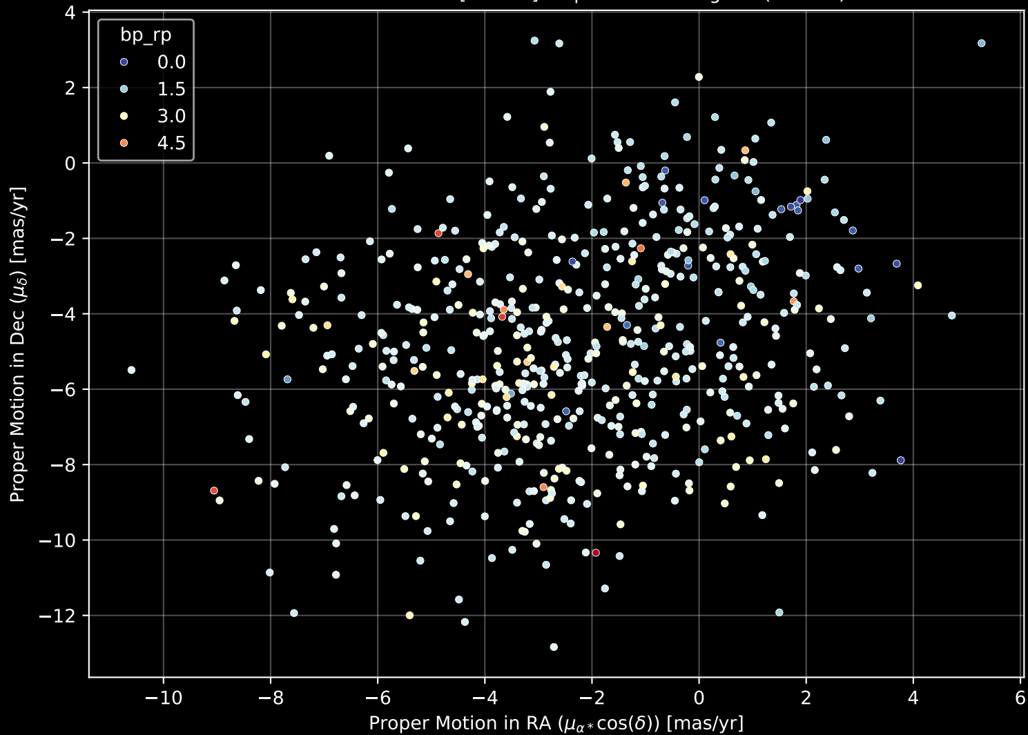
APOGEE DR17 Field: [002-04] Proper Motion Diagram (n= 584)
