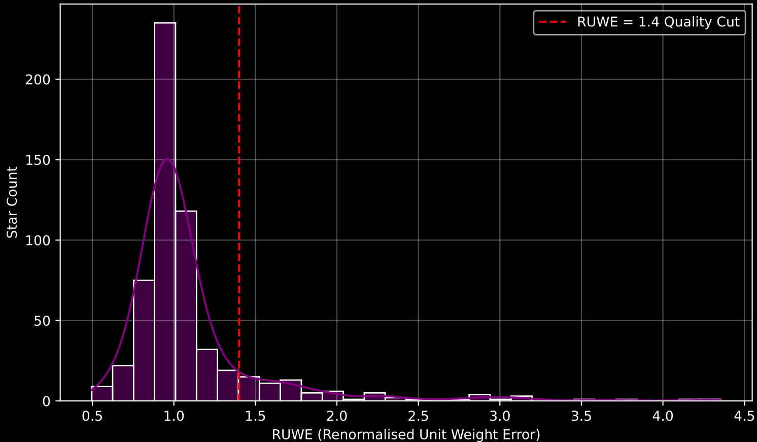
GAPOGEE DR17 Field [002-04] RUWE Distribution (n= 583)
