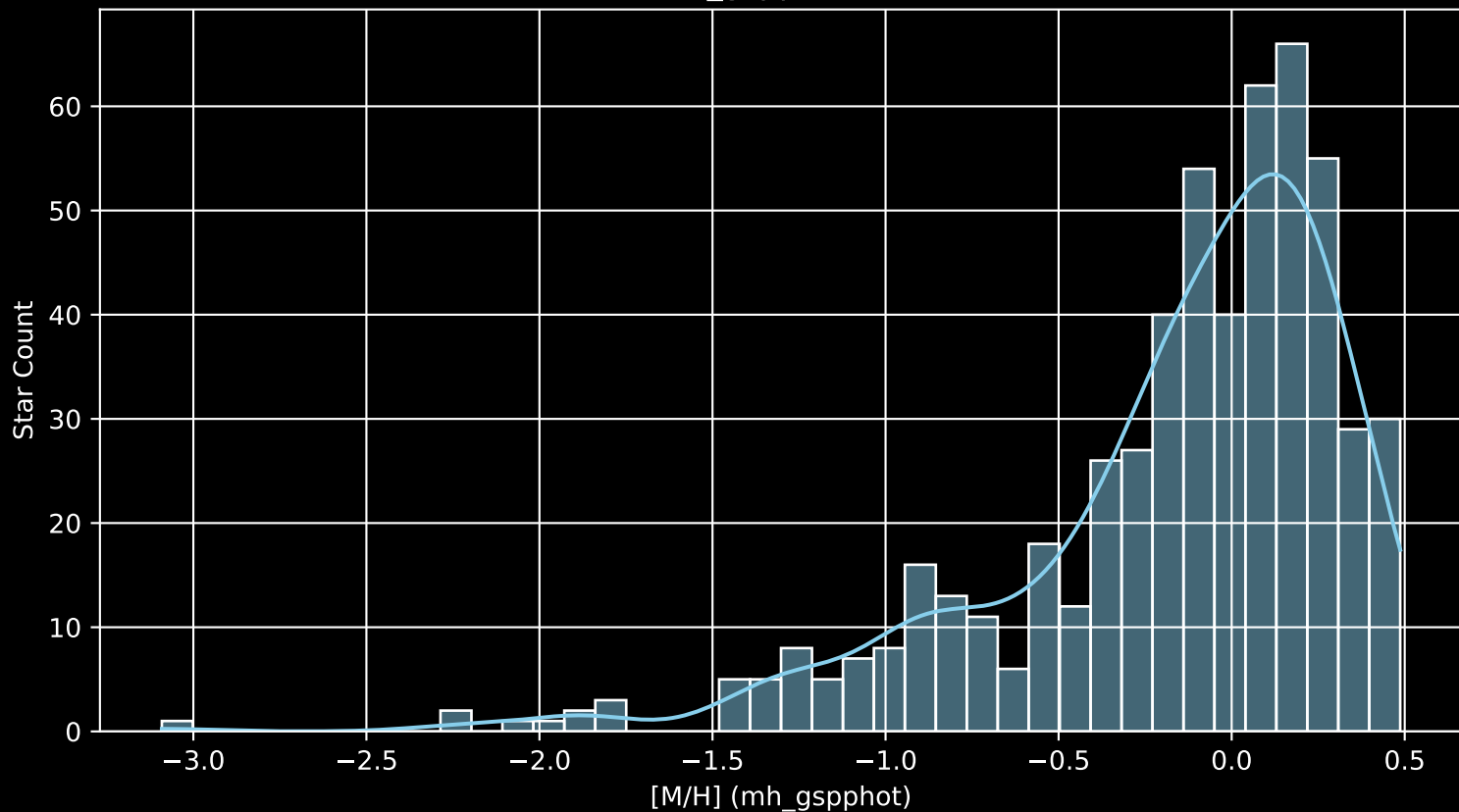
APOGEE DR17 Field: [002-04 [M/H] (mh_gspphot) (n= 553)
