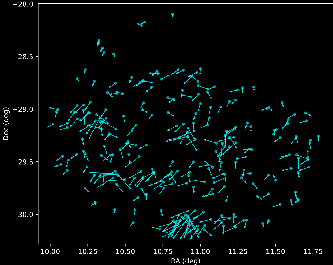
APOGEE DR17 Noise Stream Proper Motion Vectors (n=257)
