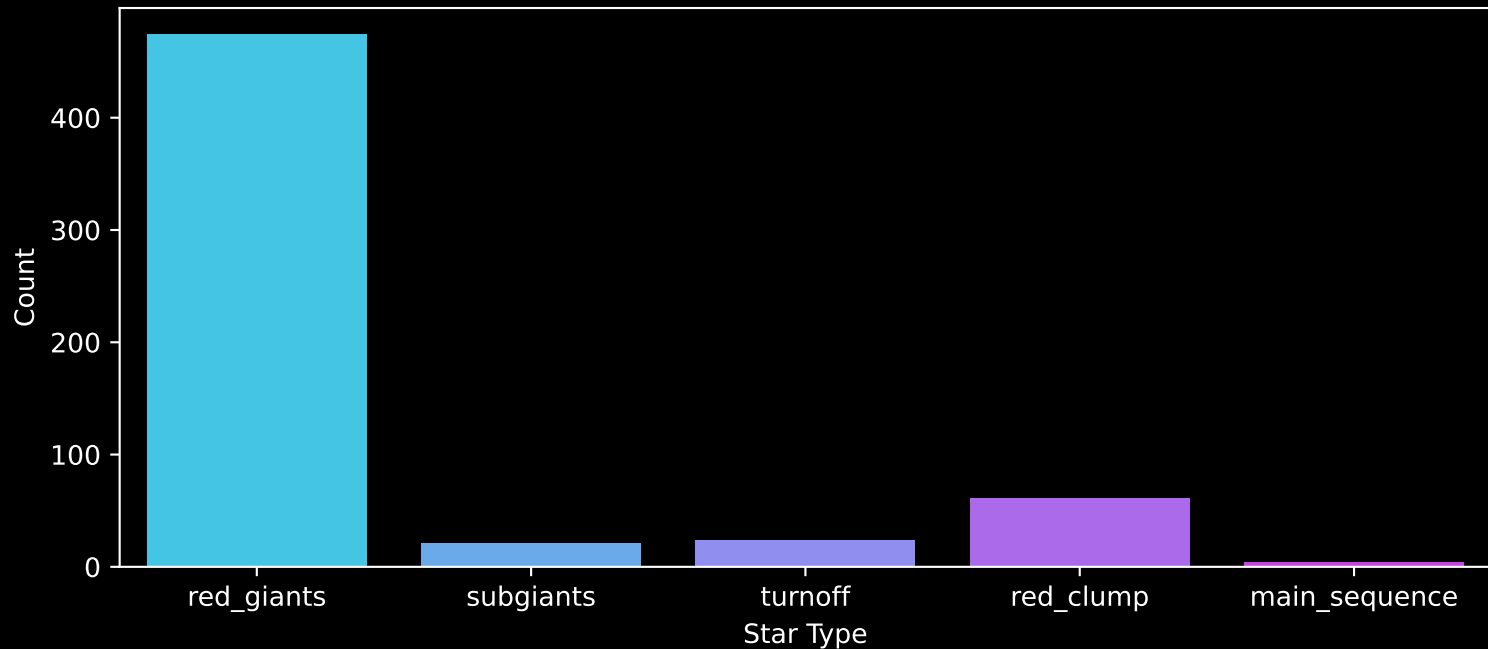
APOGEE DR17 Field: [002-04] Count plot of Star Type
