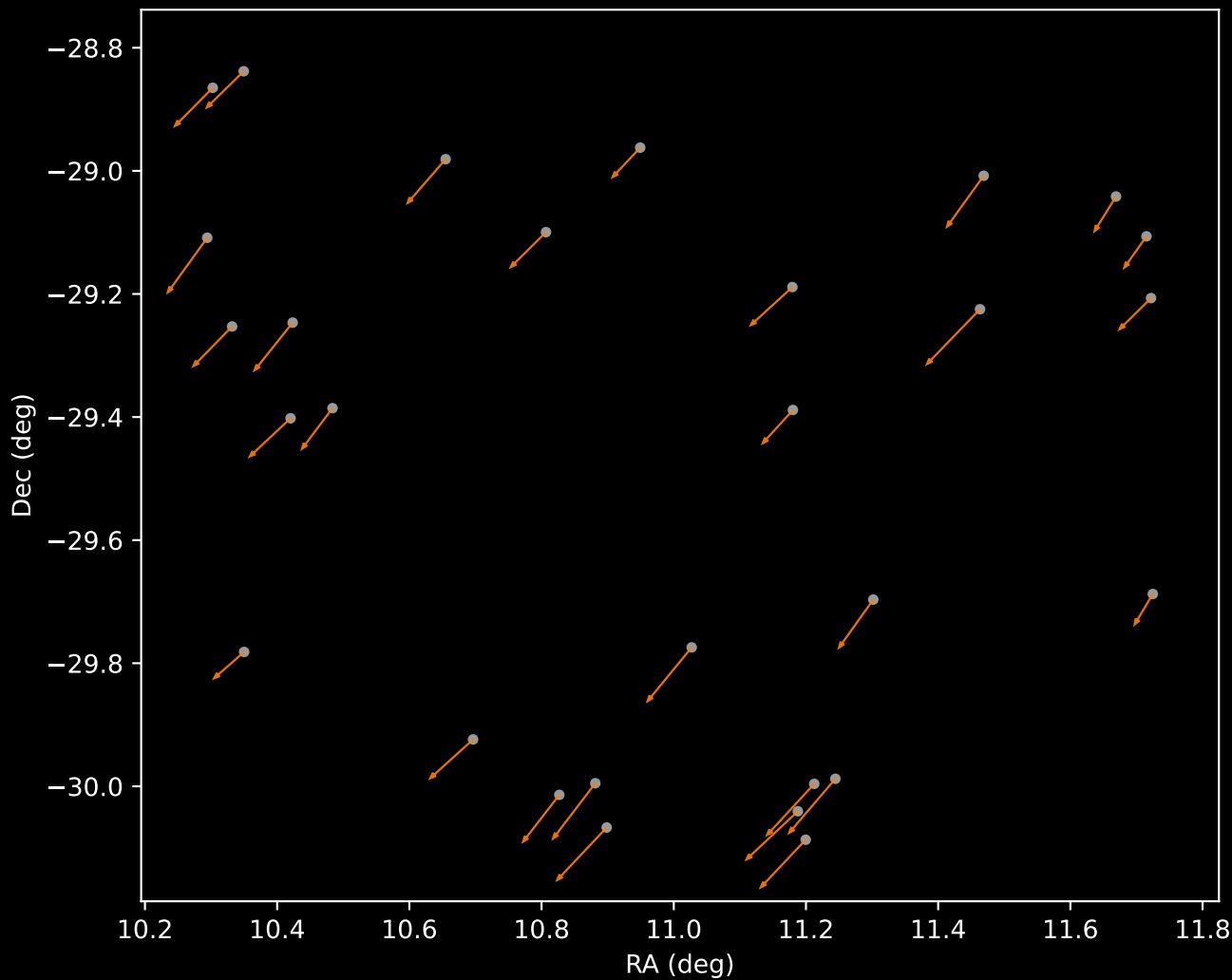
APOGEE DR17 Cluster 22 Proper Motion Vectors (n=29)
