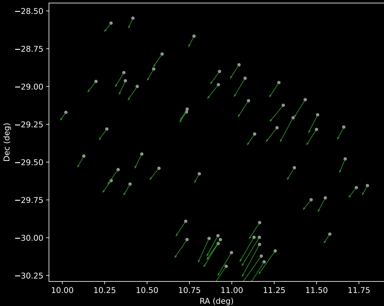
APOGEE DR17 Cluster 24 Proper Motion Vectors (n=56)
